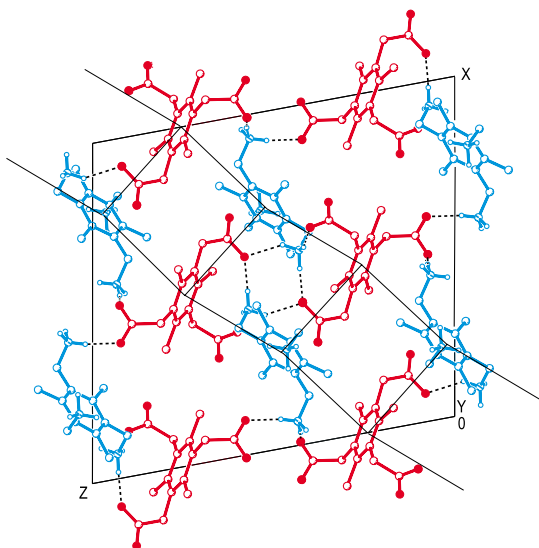
FIG. 3 Direct ionic hydrogen bonds -^+\text{NH}_3\cdots^-\text{OOC}- in the crystal structure of salt 1
